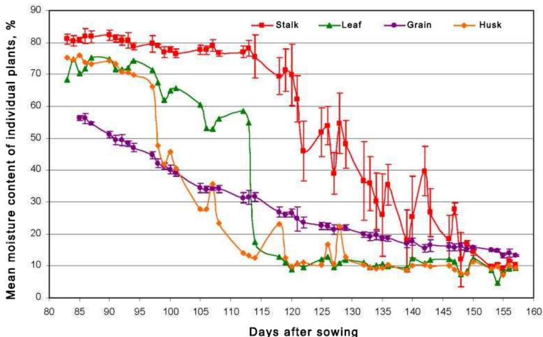
Fig. 13. Moisture distribution in overground part of a standing corn [17].
